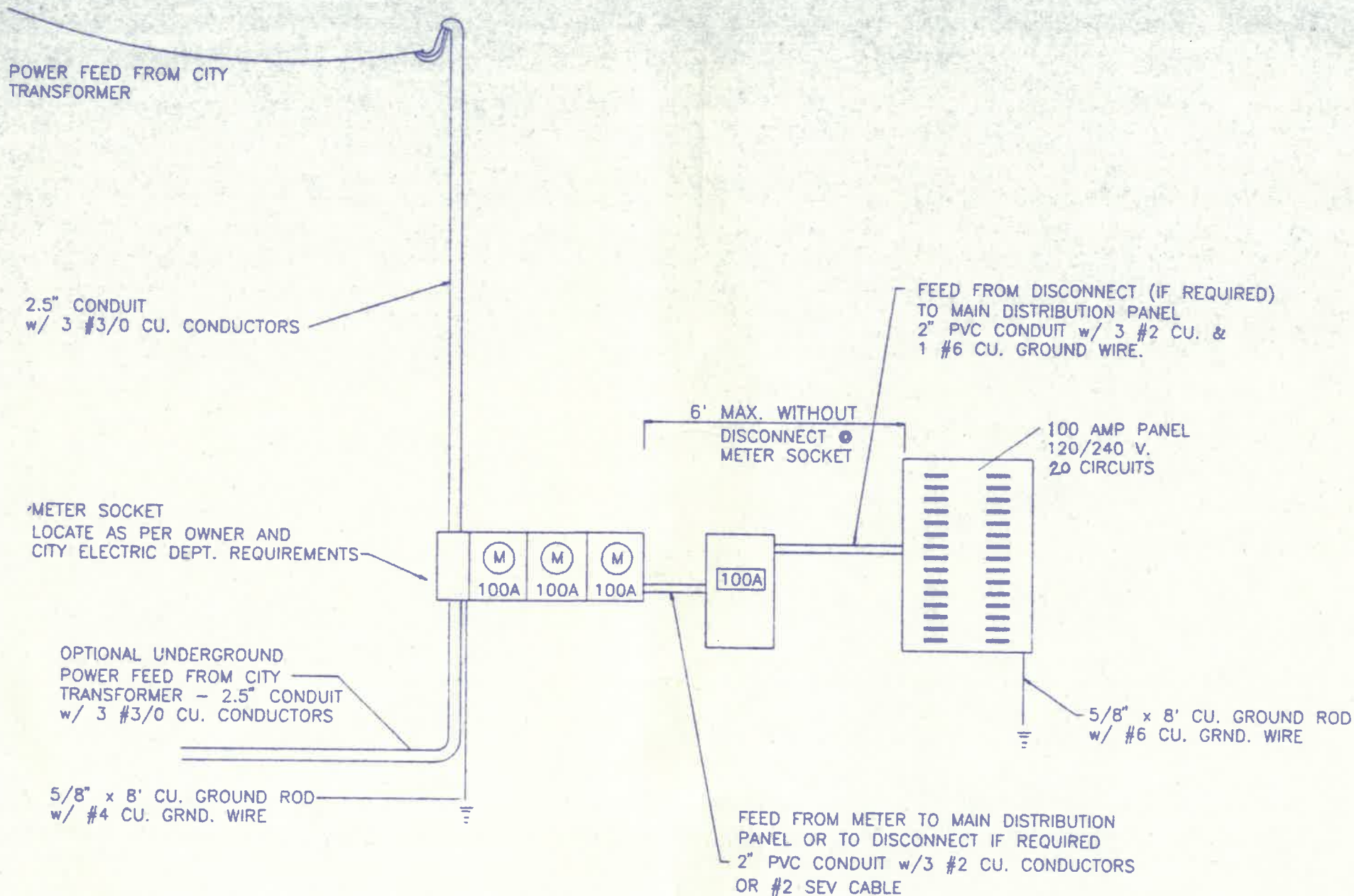
ELECTRIC RISER DIAGRAM
